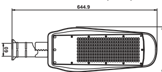
Dimension ( mm )
