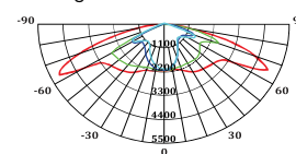
Light Distribution Curve
